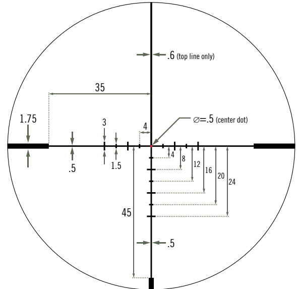
Subtensions measured in MOA. Reticle image shown for representation only.
