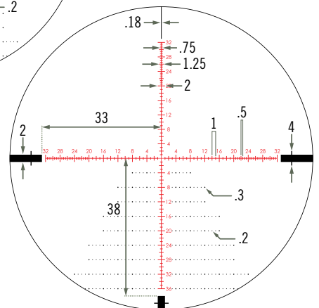
5-25 x 50 EBR-2C
