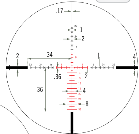
2-10 x 32 EBR-4
